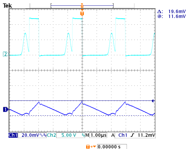
AD1510 V_{OUT} Ripple ( V_{IN}=12V ; V_{OUT}=3.3V ; I_{OUT}=0.1A )
