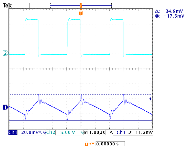
AD1510 V_{OUT} Ripple ( V_{IN}=12V ; V_{OUT}=3.3V ; I_{OUT}=3A )
